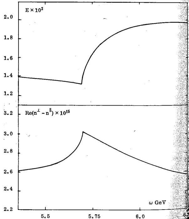
FIG. 2. E (upper part) and \text{Re}(n^\perp - n^\parallel) (lower part) as a function of \omega at \delta = 3.7 mrad.
